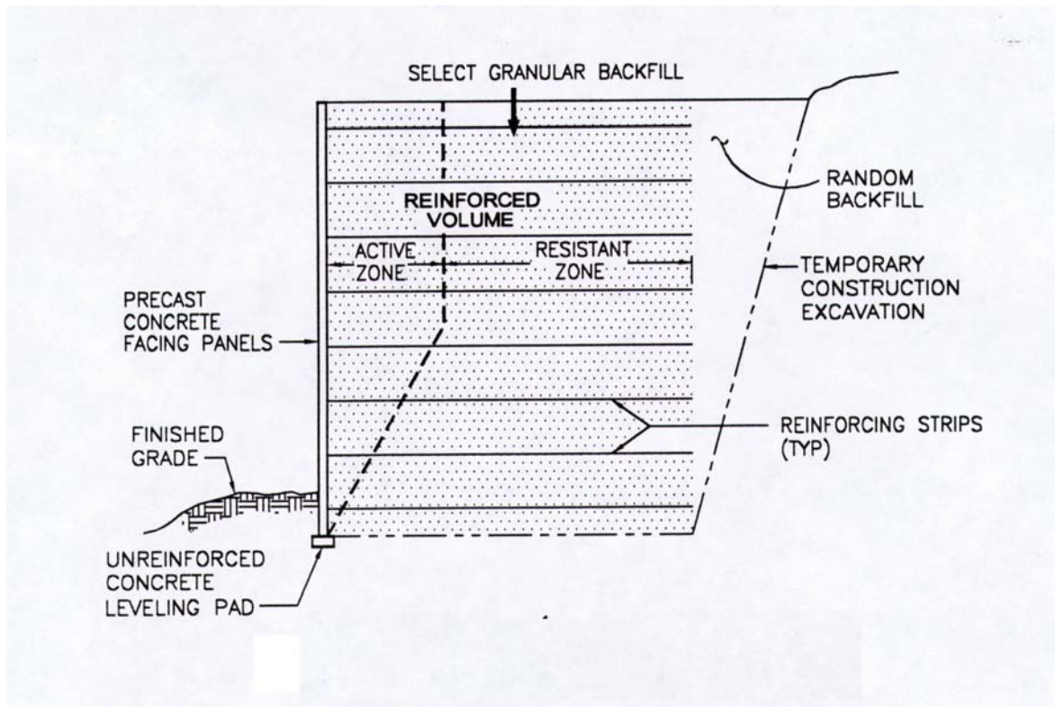
Figure 1. Typical section of a Reinforced Earth Structure.
